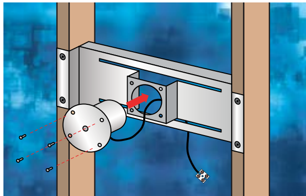
figure 3. mounting bracket attached to studs.
